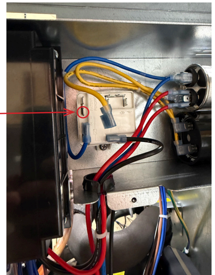
Figure 1: Incorrect Wiring
