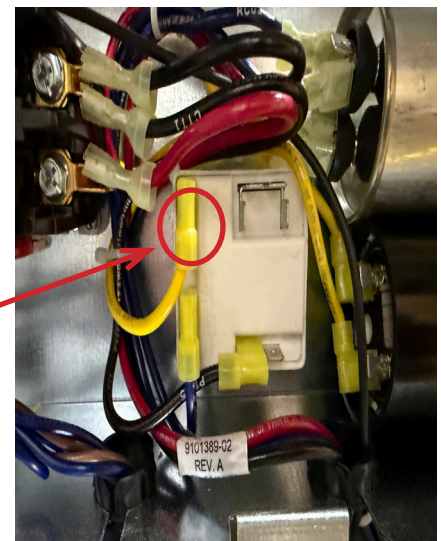
Figure 2: Correct Wiring
