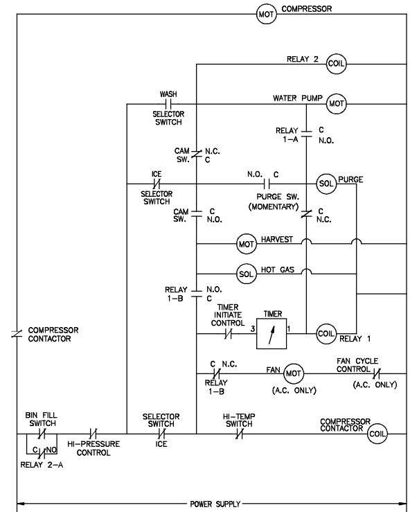
WIRING SCHEMATIC AIR & WATER (SHOWN IN TIMED PORTION FREEZE CYCLE)
